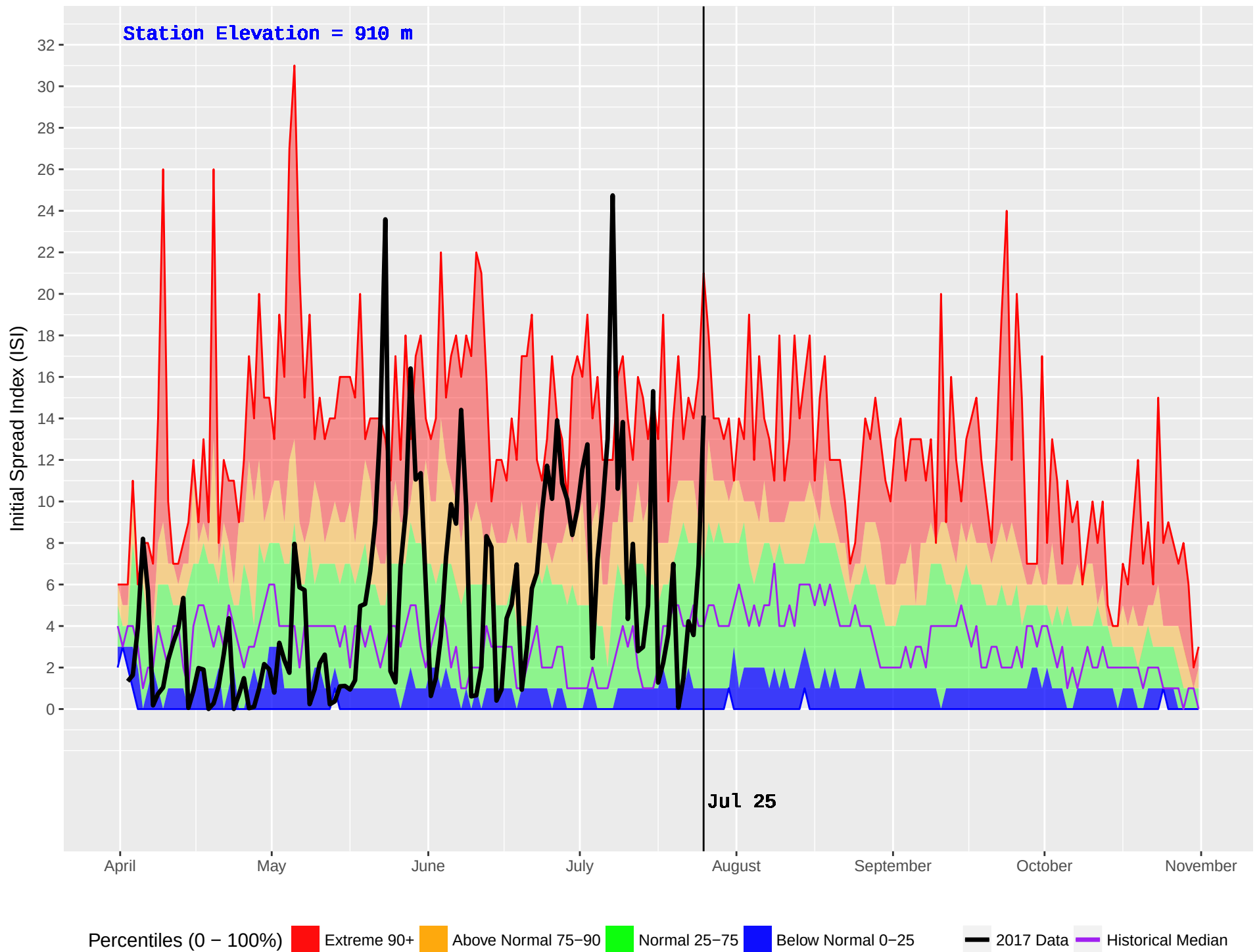
NAZKO (211) : Historical (1981–2016) and Current (2017) Noon Initial Spread Index (ISI)
